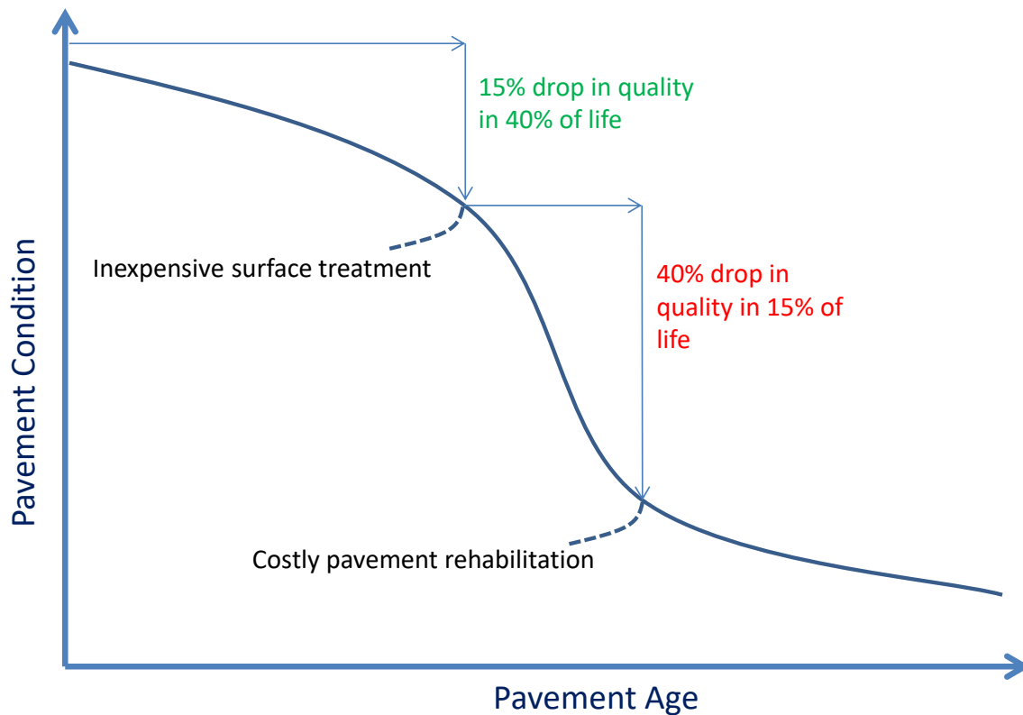
Figure 3 – Pavement Deterioration and Life Cycle Costs
