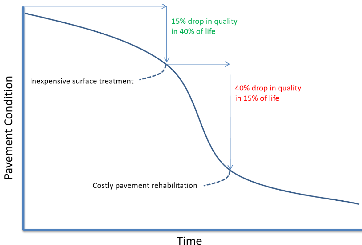
Figure 4 - Pavement Deterioration and Life Cycle Costs
